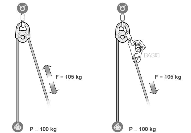
6A. Simple pulley system
