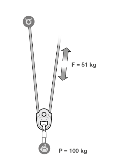
6B. 2:1 hauling system
