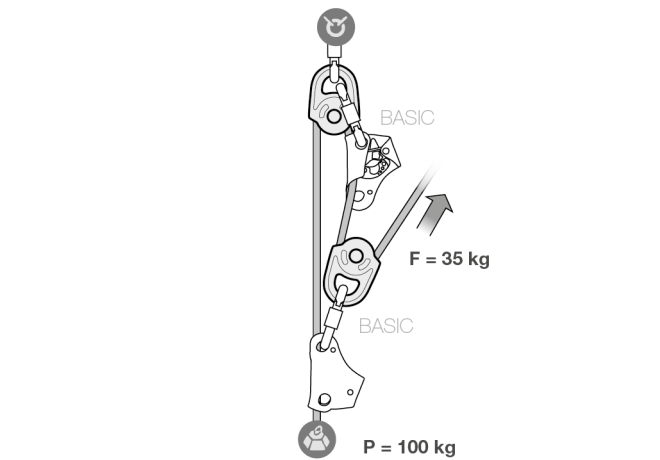
6c. 3:1 hauling system with progress capture
